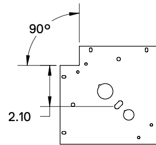
90° Bracket
