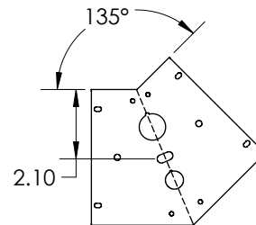
135° Bracket
