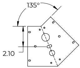
135° Bracket
