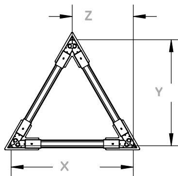
HANGING KIT ATTACHMENT POINTS
