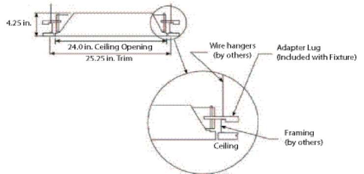
RF2x4 Dimensions
