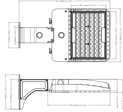
Wall Mount (150-200W)
