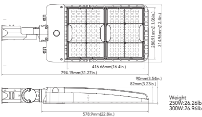
Slipfitter Mount (300W)
