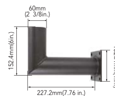
90° Wall Mount Bracket with 2-3/8" O.D. Tenon NO. WMVD Finish: Dark Bronze USE: The 90° wall mount bracket with 2-3/8" tenon attaches an MESTER floodlight to almost any surface: wall, roof, or wood pole. Provides wiring access and a built-in 2-3/8" O.D. tenon to mount a fixture with our adjustable slipfitter. Suggested 3/8" diameter bolts for mounting. Mounting holes are spaced 3-1/4" apart.
