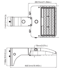
Slipfitter Moun (70-105W)
