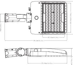
Slipfitter Moun (150-200W)
