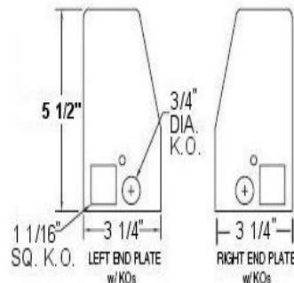
741 Series End Plate View
