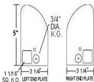
74 Series End Plate View
