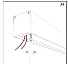
Wire the channel and attach to the surface with screws.
