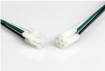
Wiring harnesses are provided in continuous run fixtures designated by -B, -J, -E for beginners, joiners and Enders. See page 193 for options.
