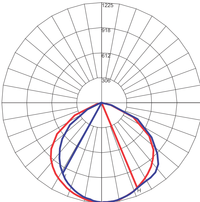
Maximum Candela = 1224.567 Located At Horizontal Angle = 1, Vertical Angle = 3 H - Horizontal Axial Candela V - Vertical Axial Candela
